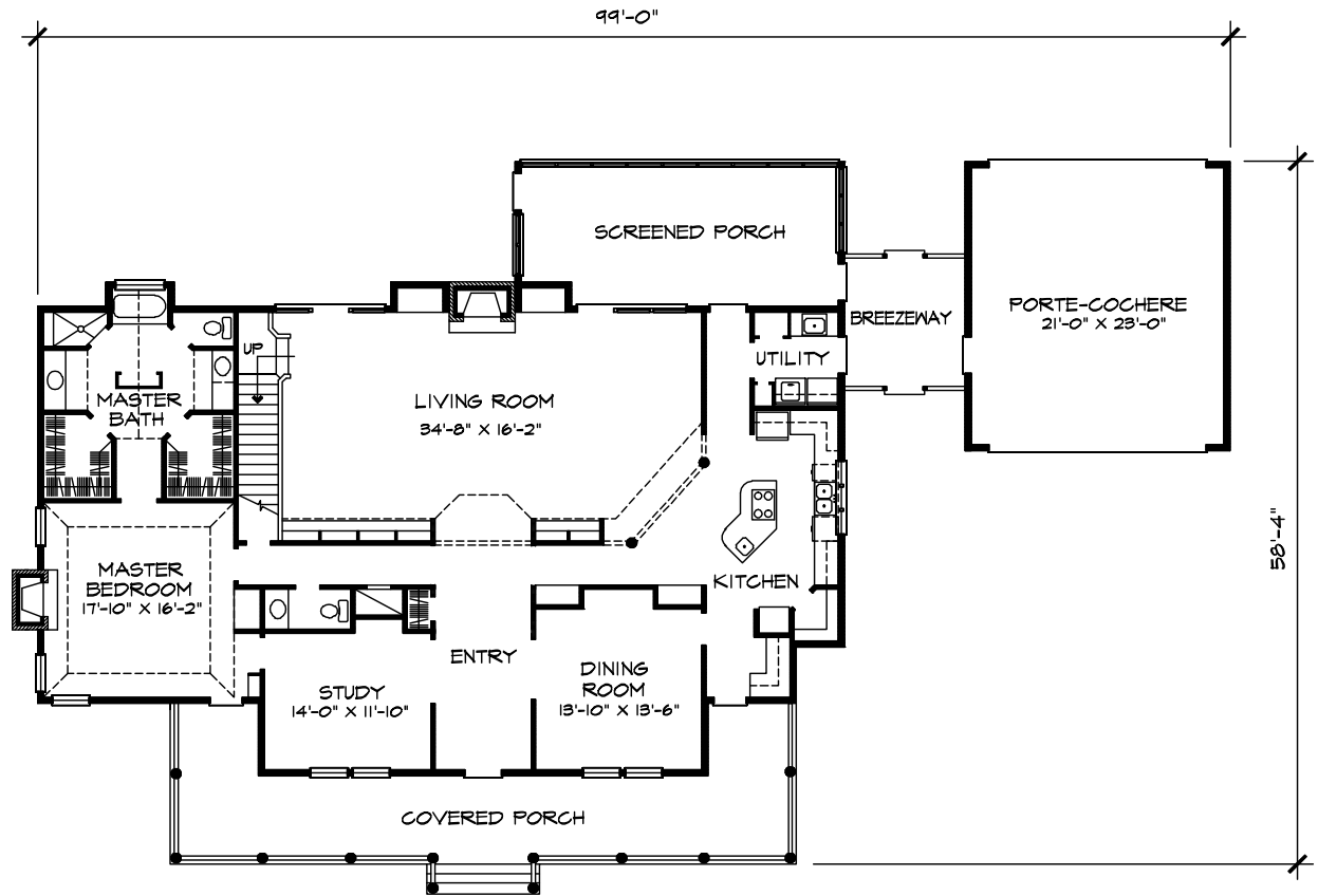
FIRST FLOOR
