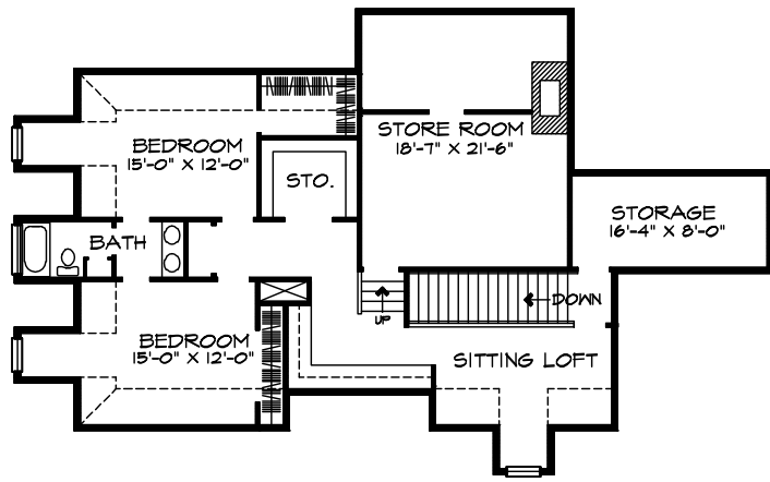
SECOND FLOOR
