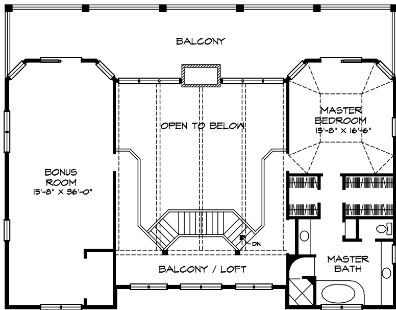
SECOND FLOOR
