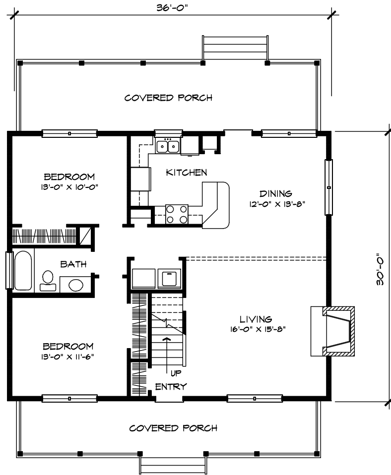
FIRST FLOOR
