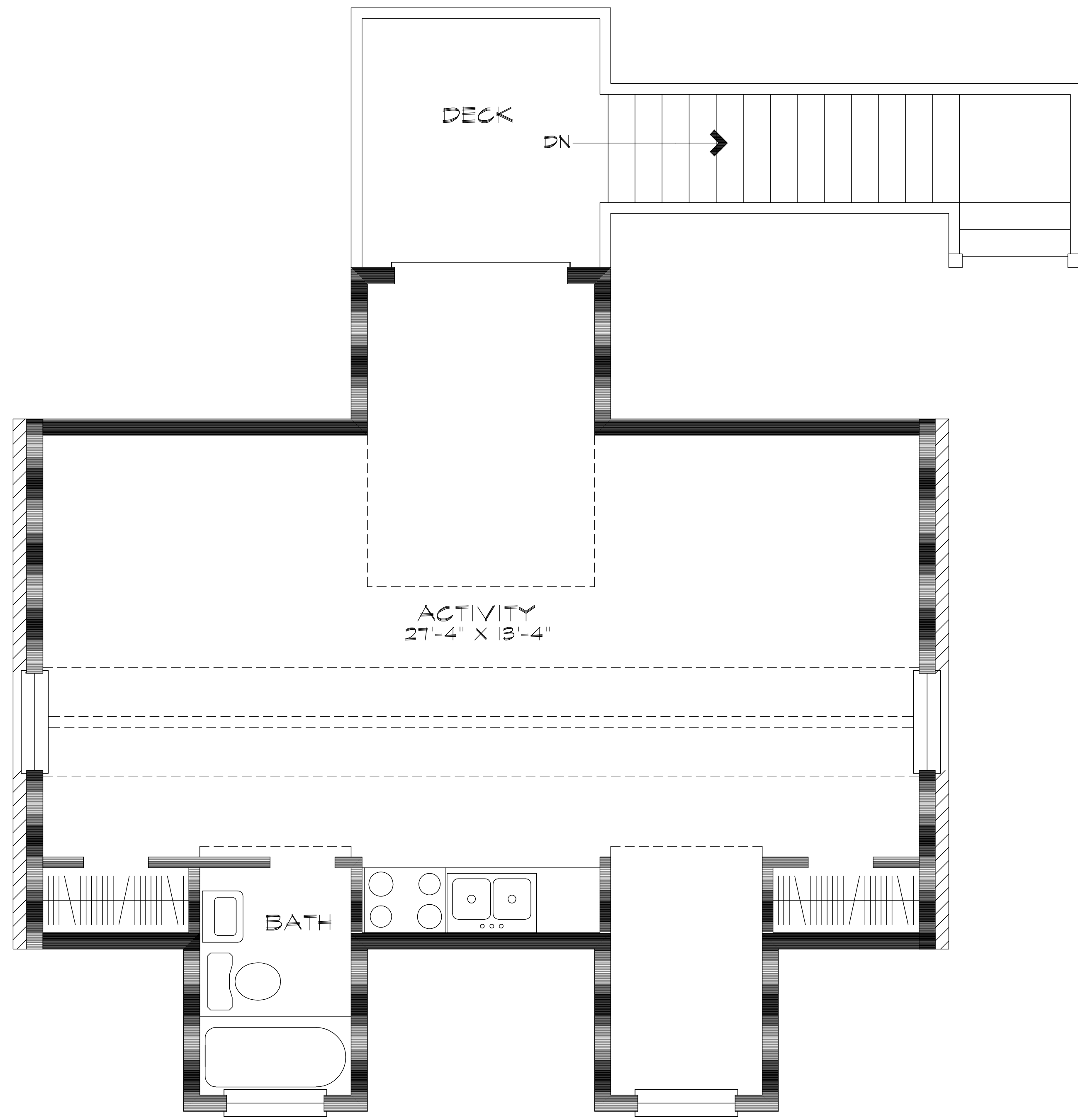
SECOND FLOOR
