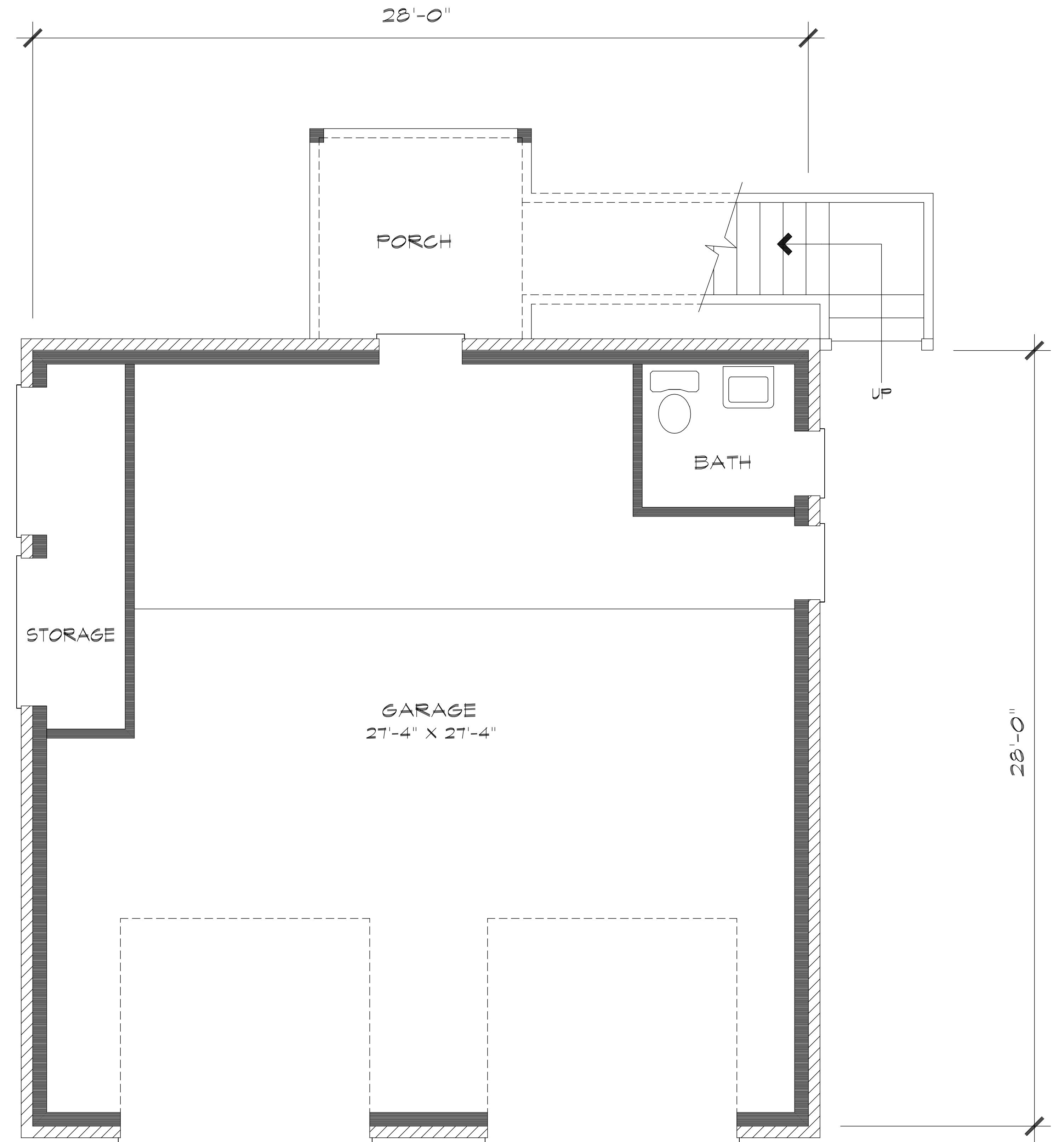
FIRST FLOOR
